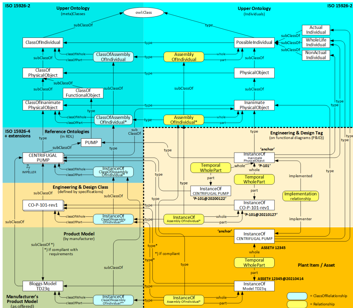
Figure 7 – Example of interrelationships between classes and individuals
