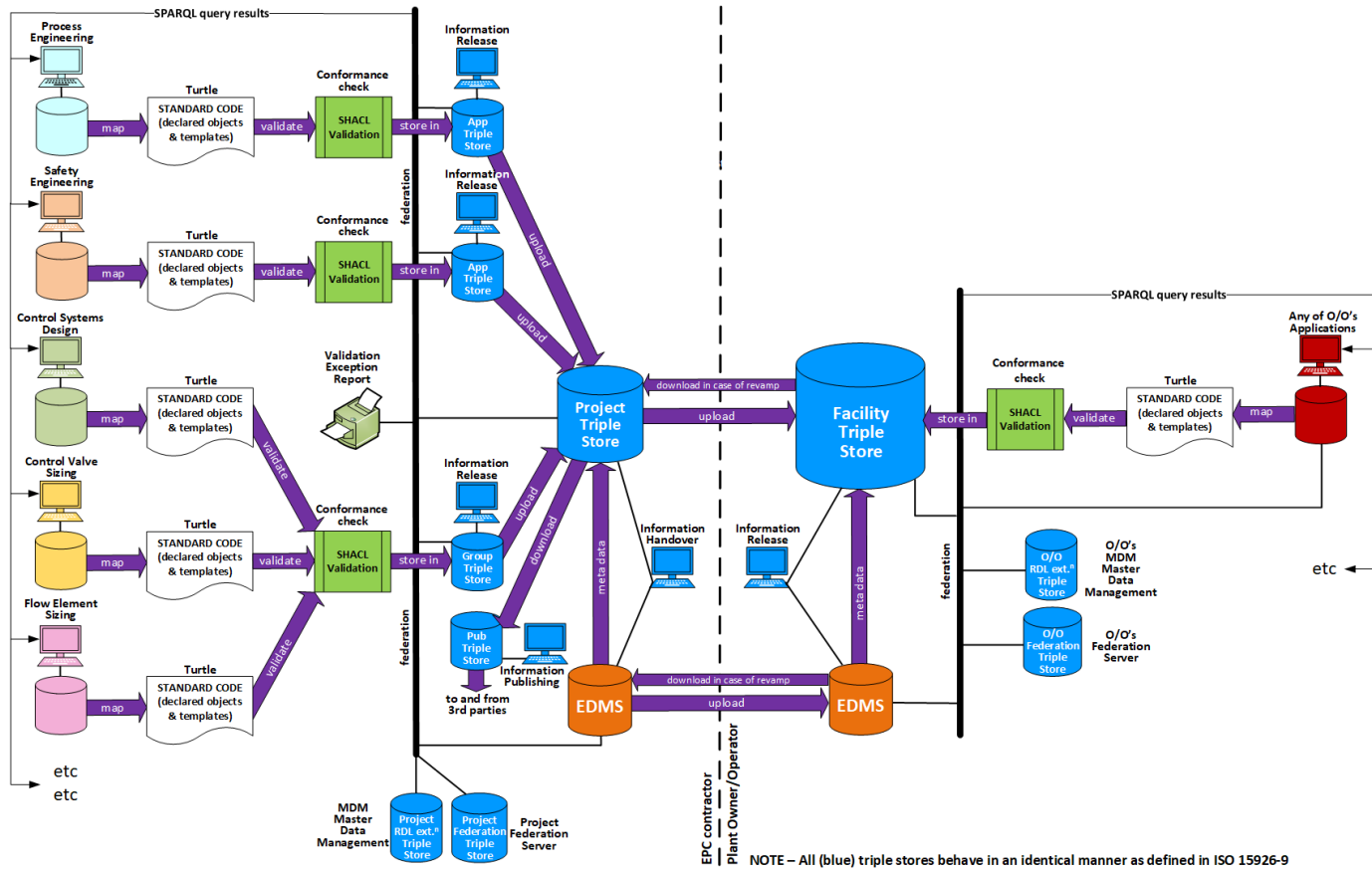
4i – ISO 15926 Information Integration Infrastructure
