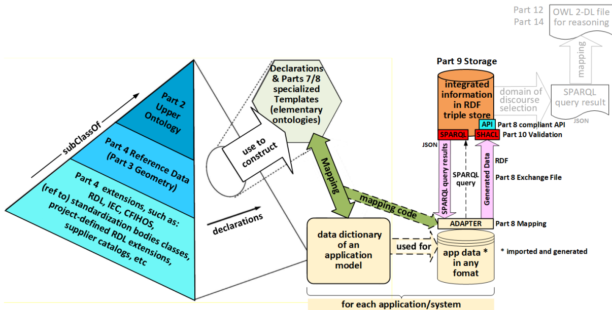
Figure 21- Architecture of ISO 15926
