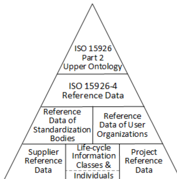
Figure 22 - the ISO 15926 global taxonomy
