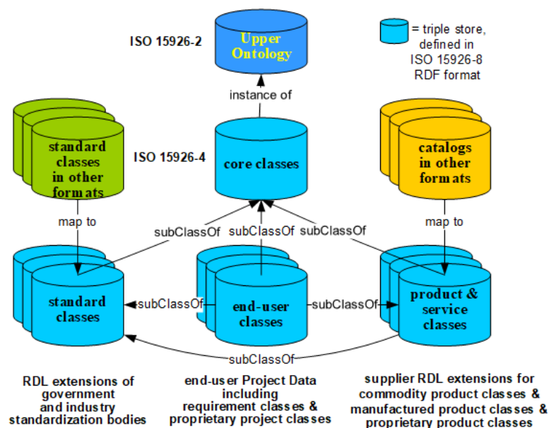
Figure 19 – Reference Data Library and its extensions
